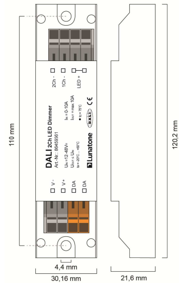
Geometrie 10A and 16A
